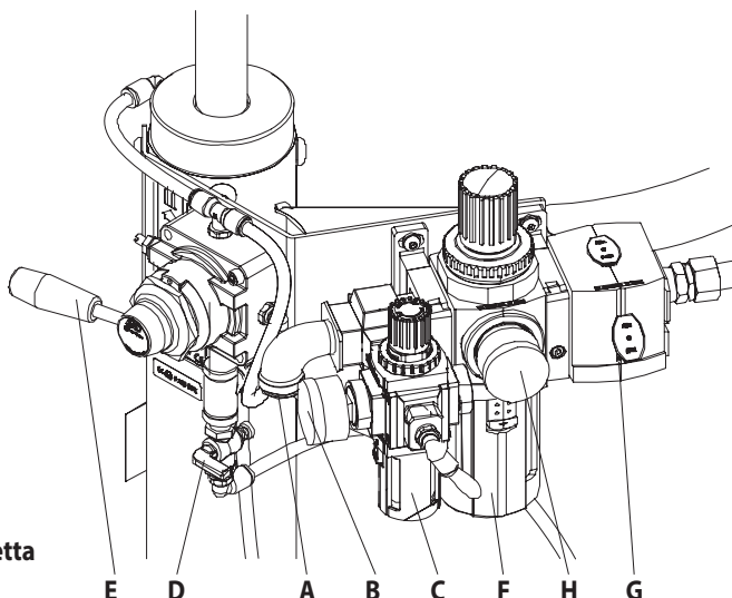
Modelli RM552H-CXX-XX
