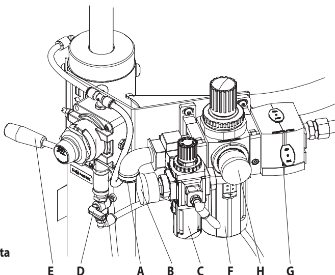
Modele RM552H-CXX-XX
